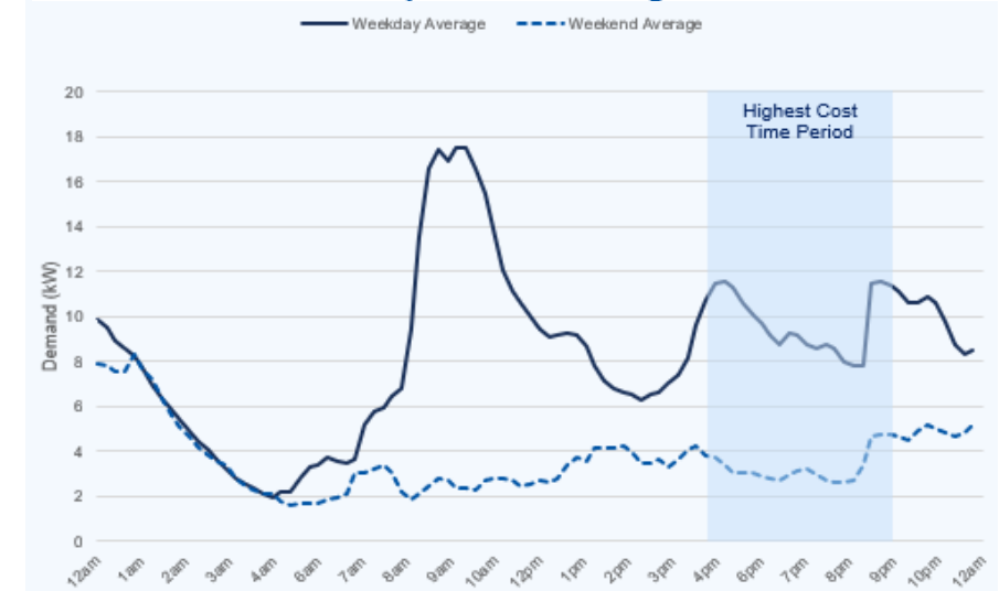
Figure 203. SDG&E PYDFF Program Weekday and Weekend Daily Average Loads for PTD Sites from September 2023 through November 2023
