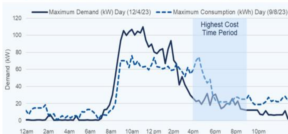
Figure 235. SDG&E Schools Pilot Highest Demand and Consumption Days Load Curve
