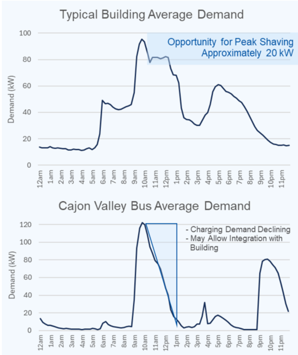
Figure 256. V2G Pilot Building and Bus Charging Load Curves
